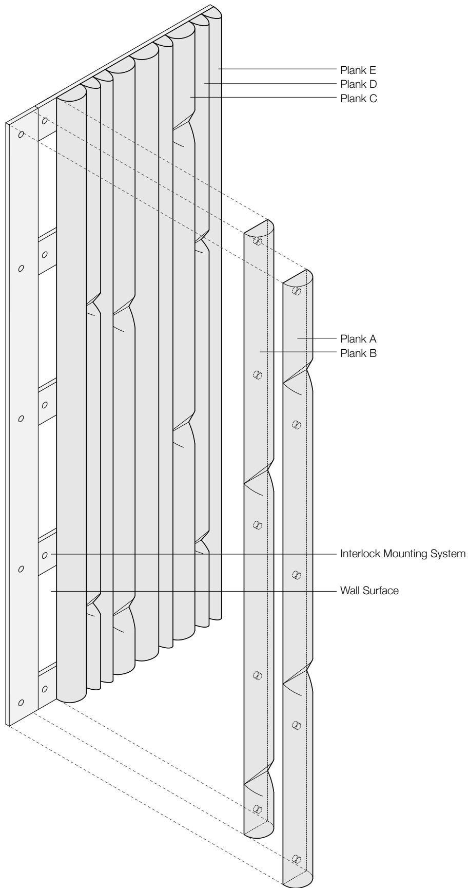
Exploded Axonometric
