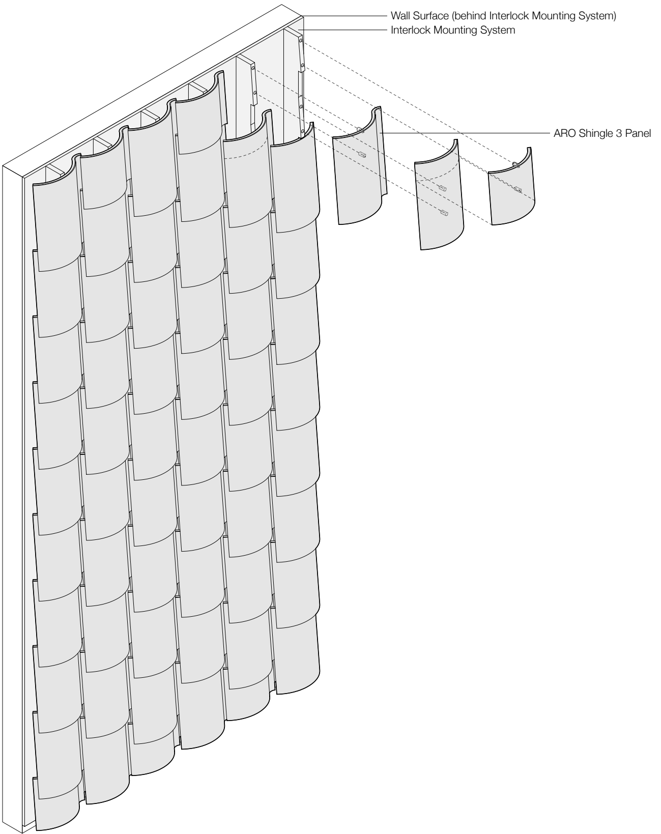
Exploded Axonometric
