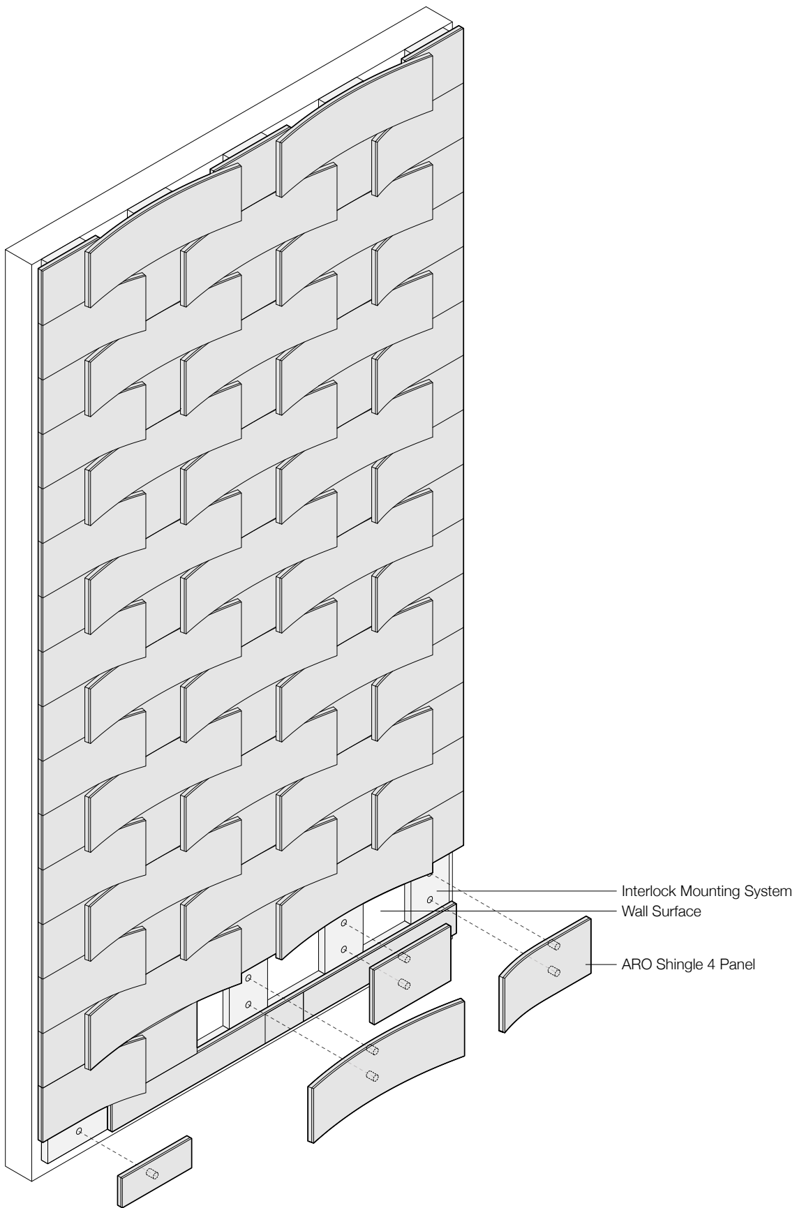
Exploded Axonometric
