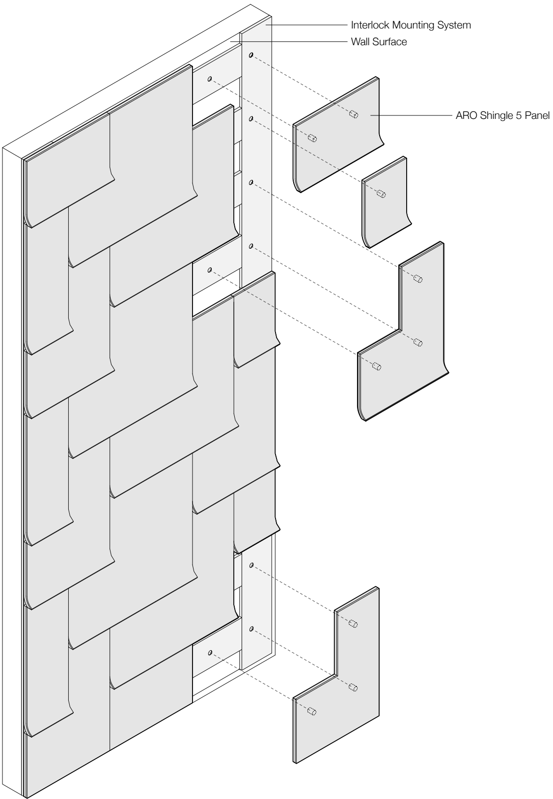
Exploded Axonometric
