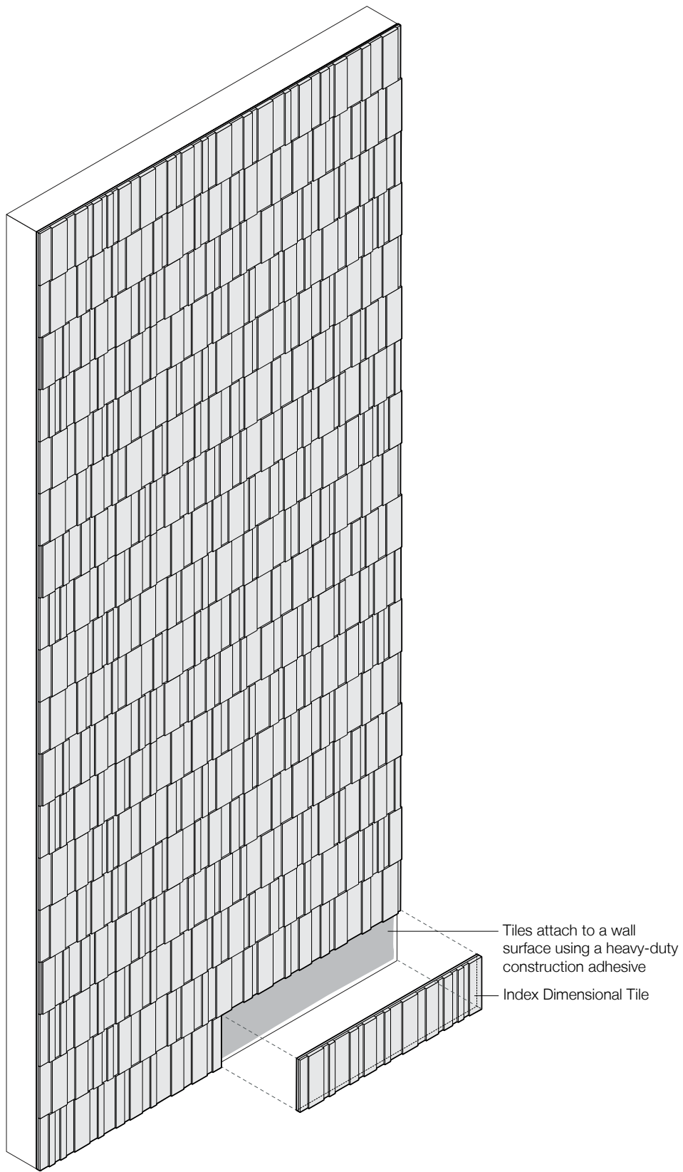
Exploded Axonometric Standard Tile Size Shown
