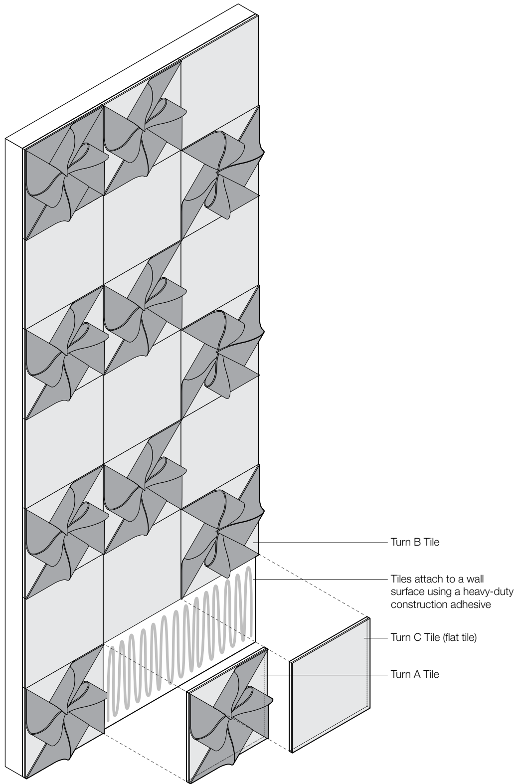
Exploded Axonometric
