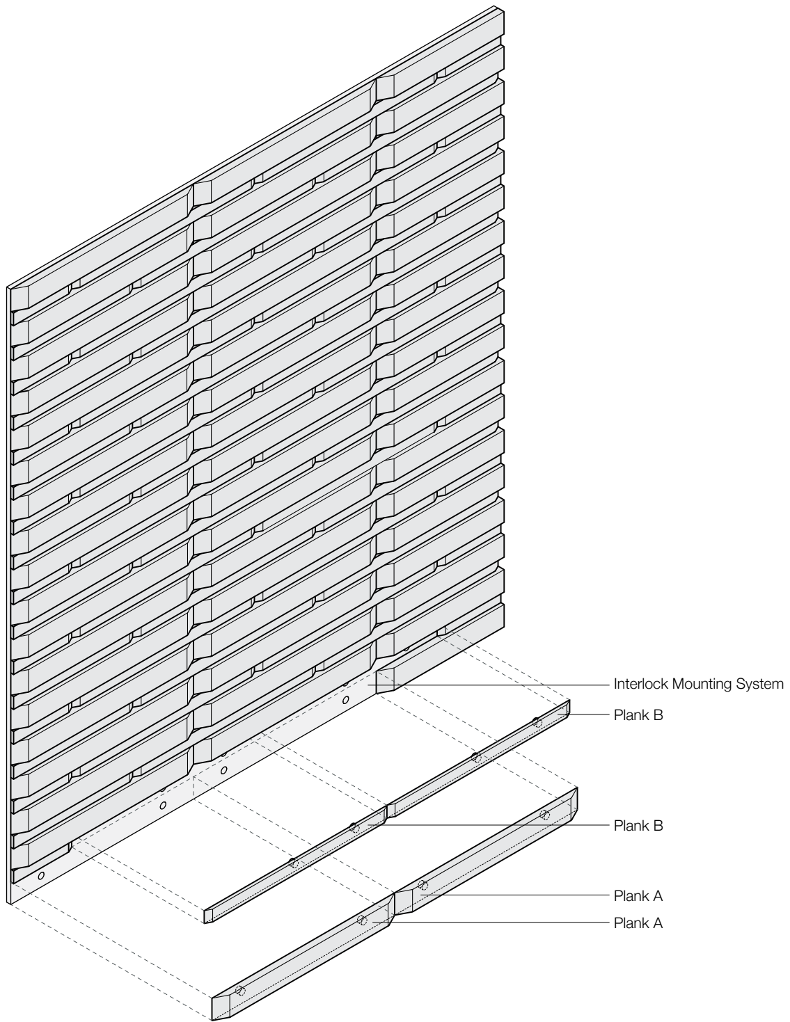
Exploded Axonometric
