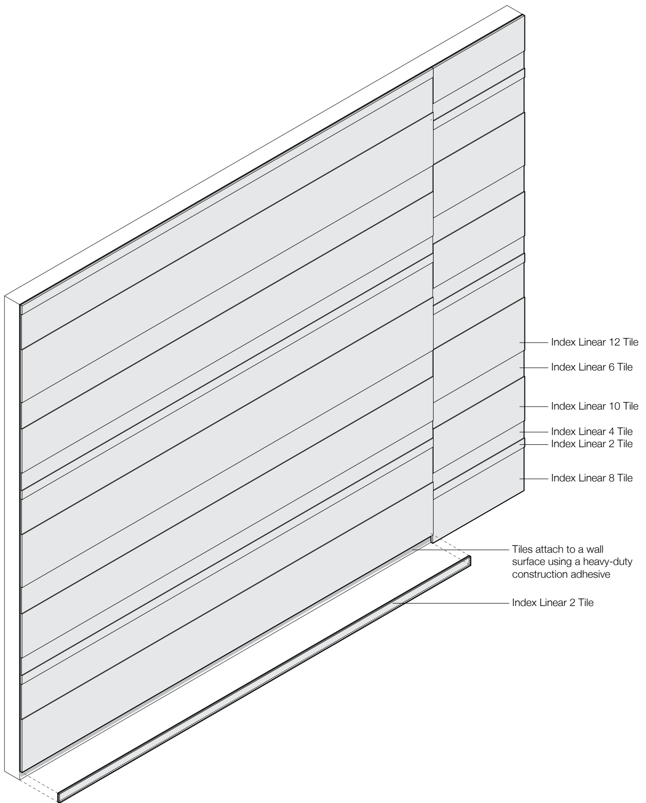
Exploded Axonometric Six Distinct Tiles in Standard Pattern
