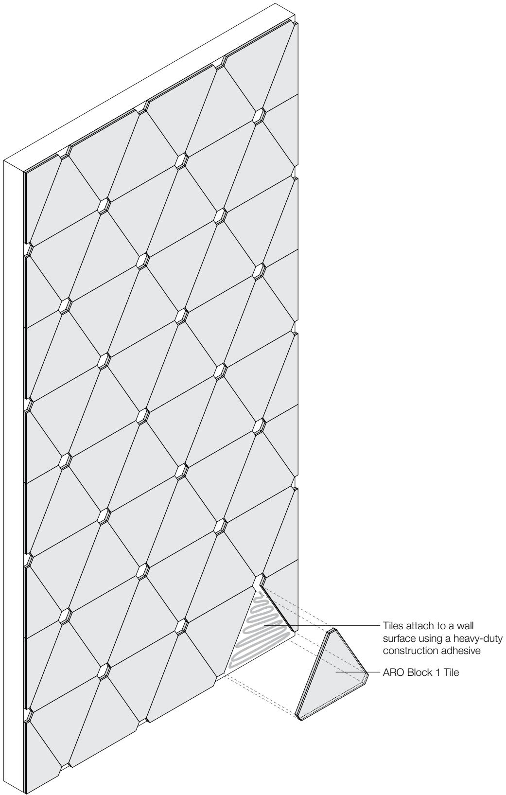
Exploded Axonometric
