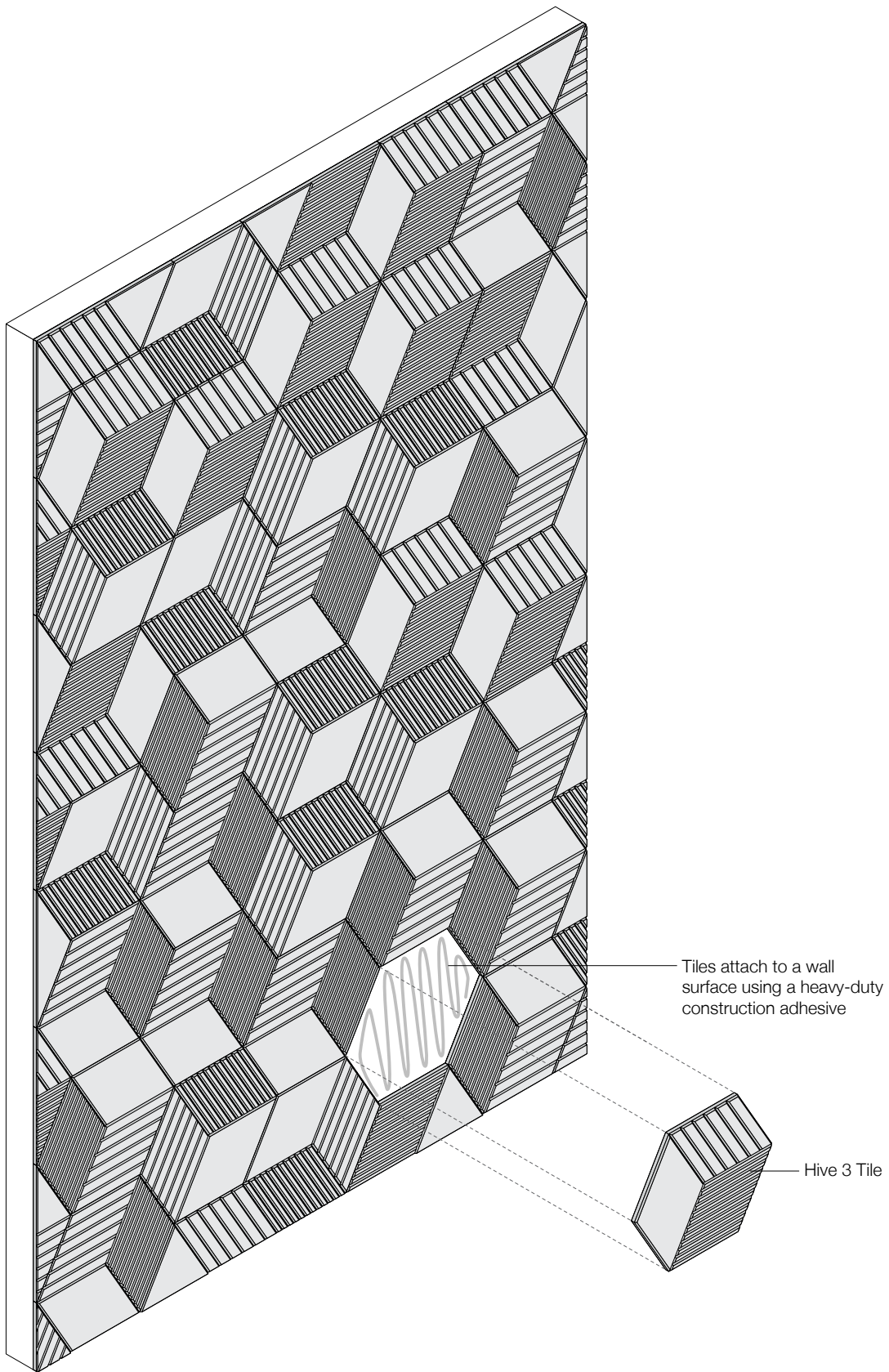
Exploded Axonometric
