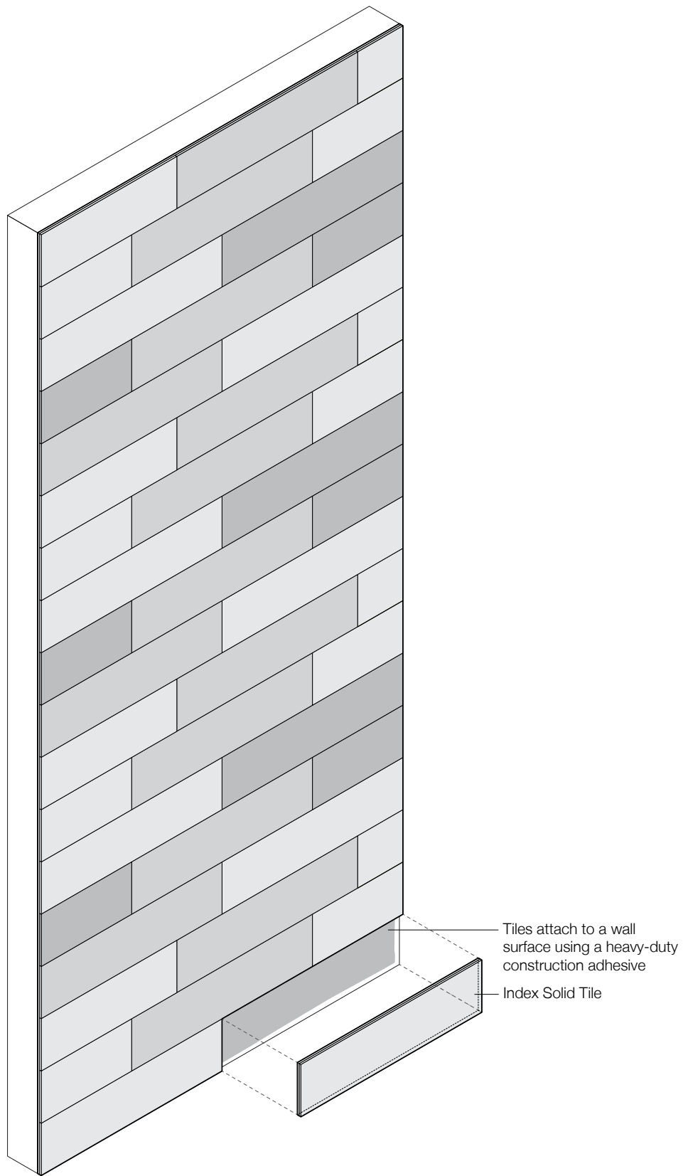
Exploded Axonometric
