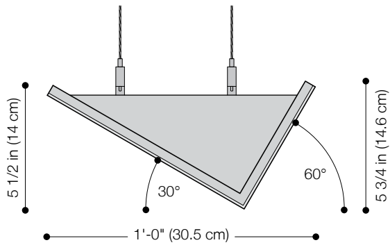
Side Elevation
