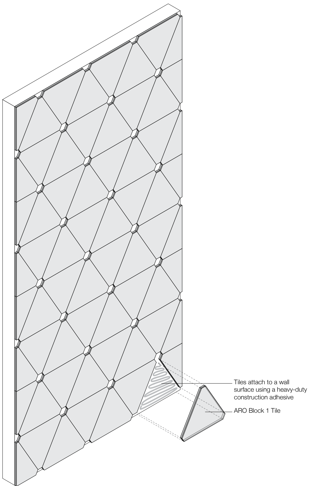
Exploded Axonometric
