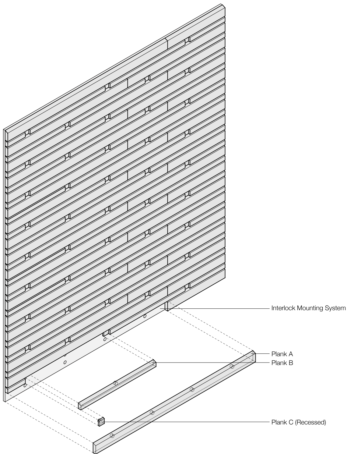
Exploded Axonometric
