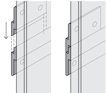
15 Slide Panel down to engage Wall and Panel Z-Clips
