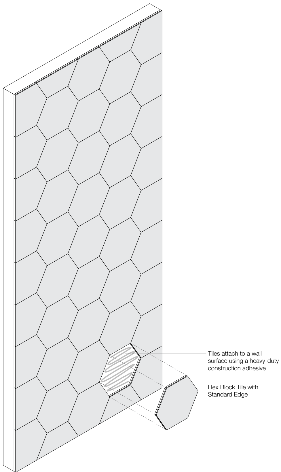
Exploded Axonometric
