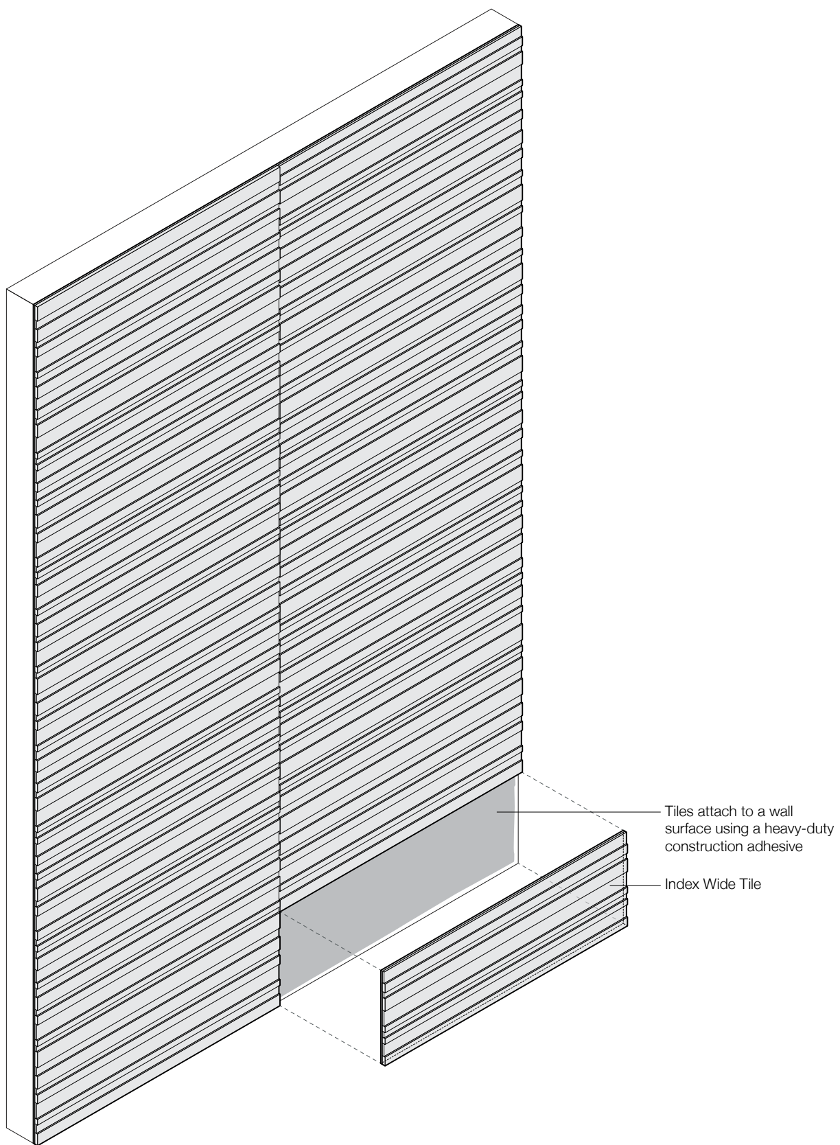
Exploded Axonometric
