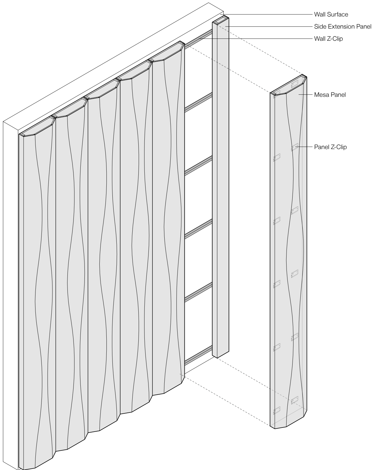
Exploded Axonometric
