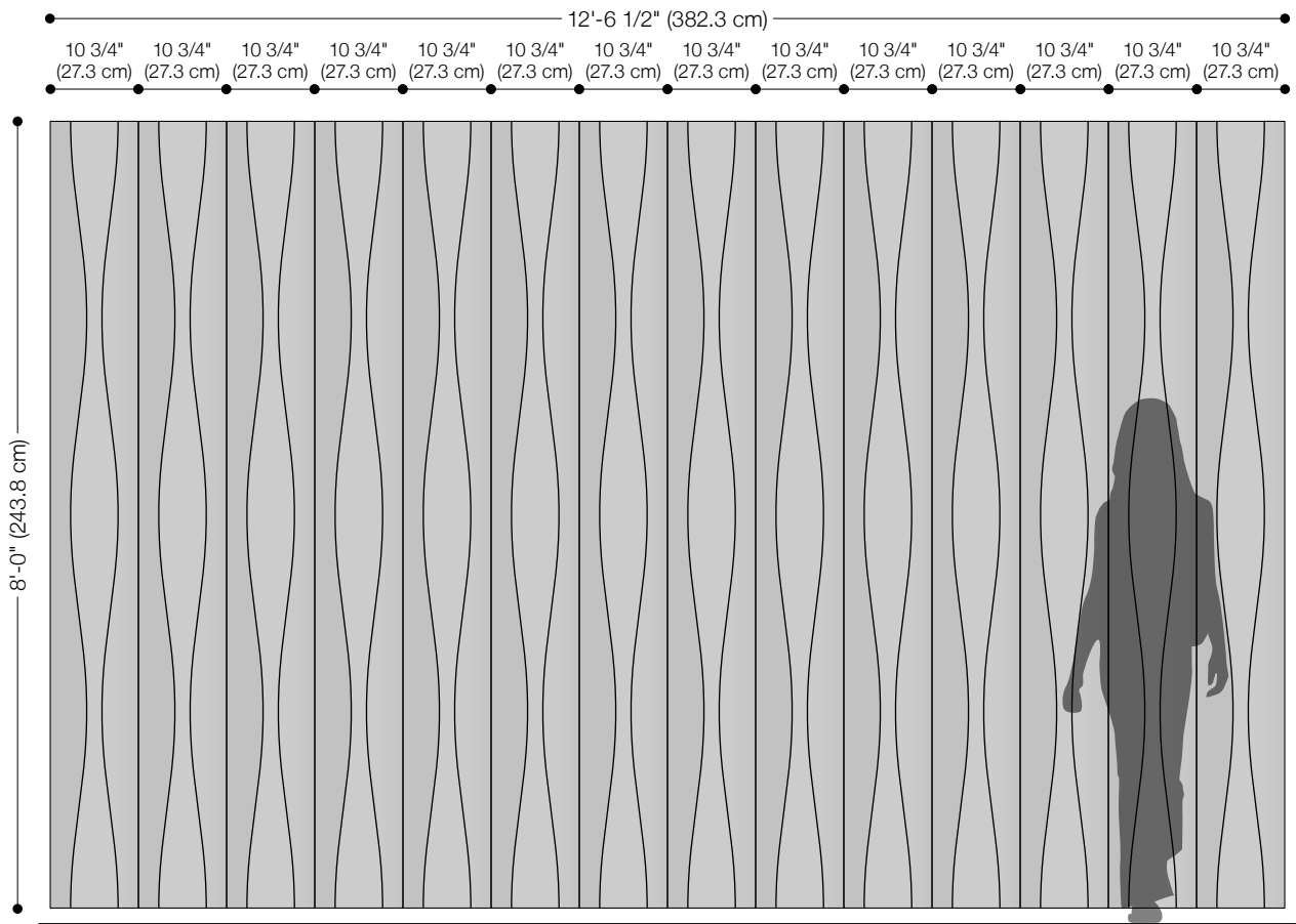
Front Elevation
