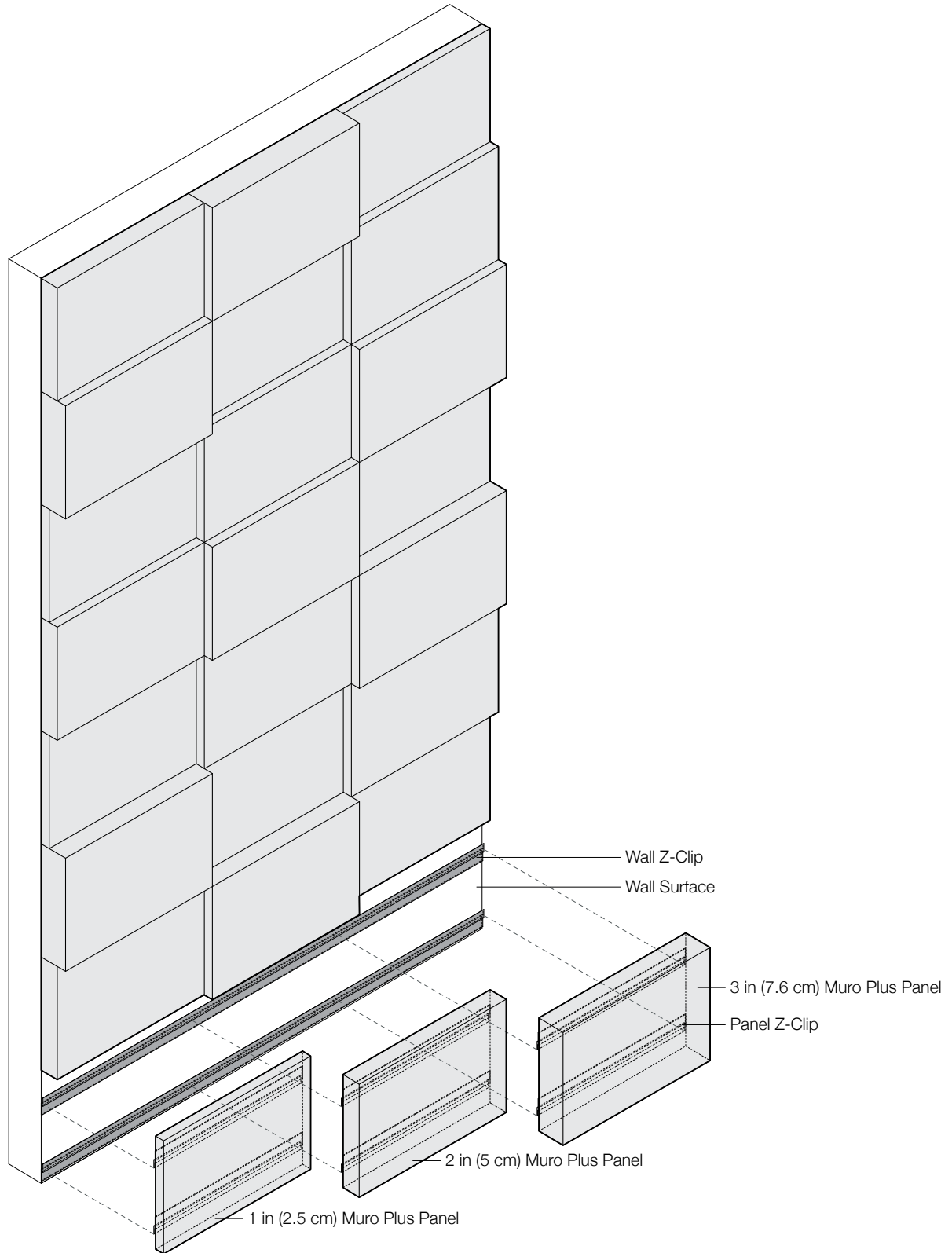
Exploded Axonometric Three Distinct Panel Thicknesses
