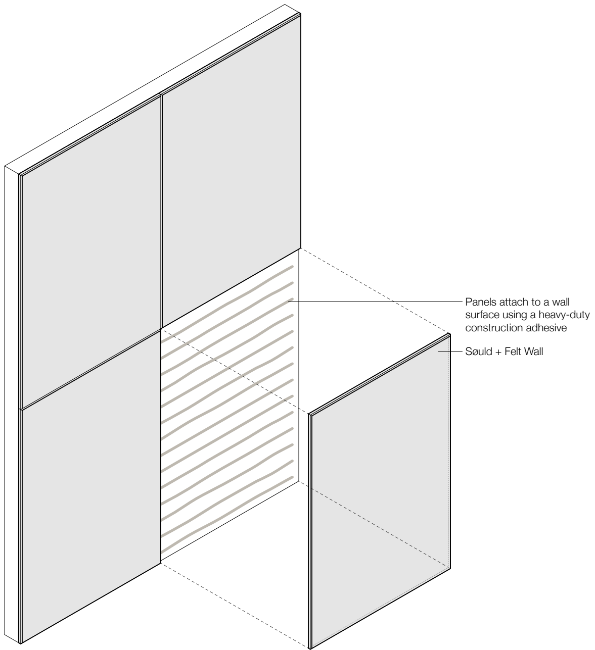
Exploded Axonometric
