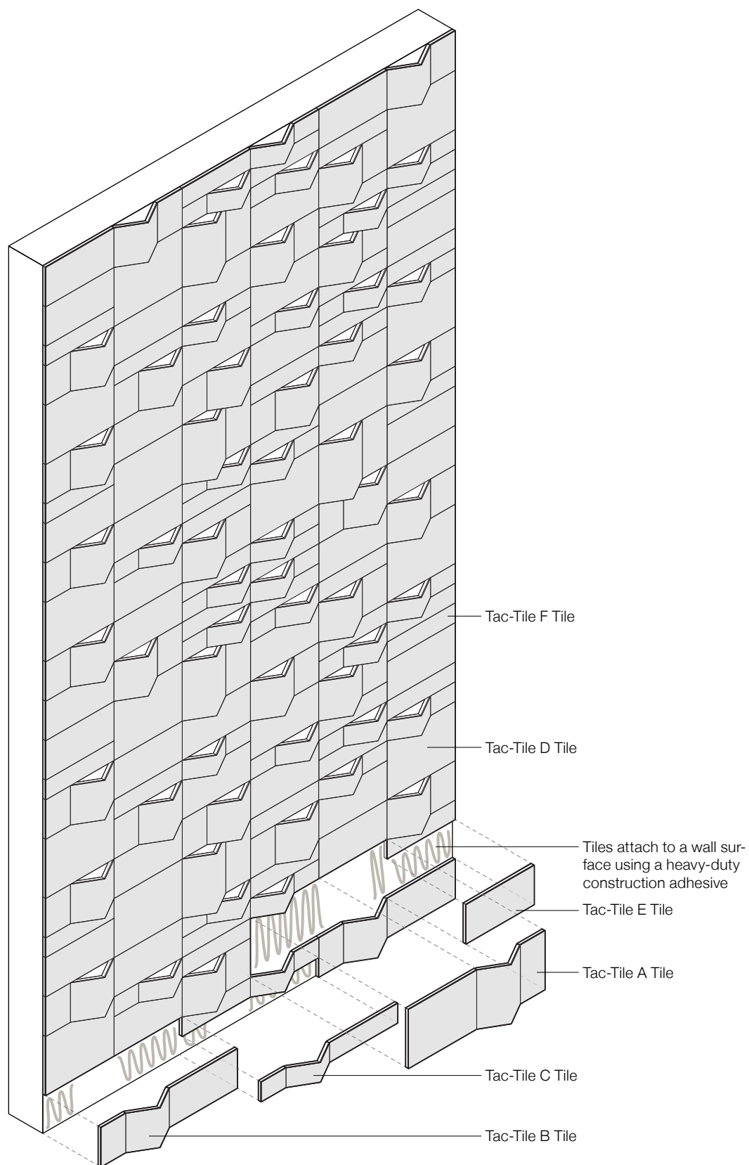
Exploded Axonometric
