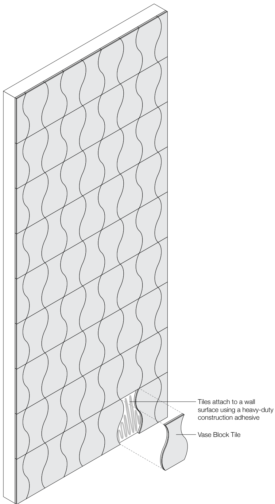
Exploded Axonometric
